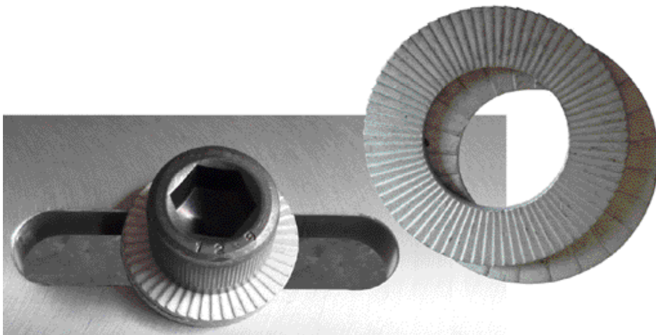
Rondelles "LOCK"
